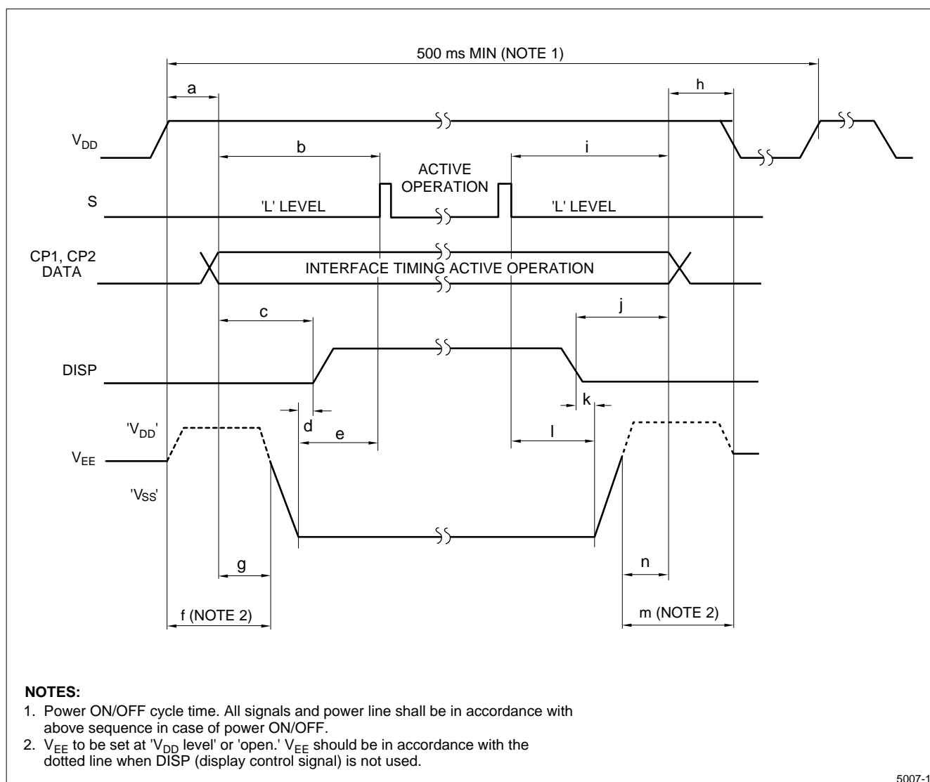
Figure 14. Supply Voltage Sequence Condition
