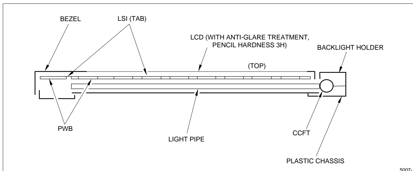
Figure 1. LM64P839 Construction
